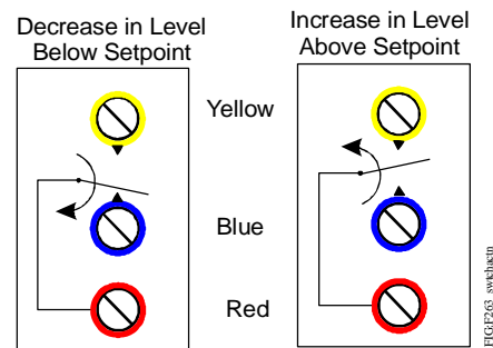
Figure 4: F263 Float Switch Action
